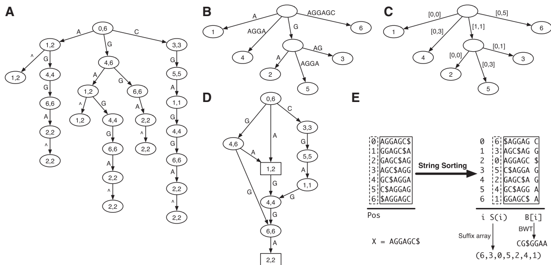
Figure 1: Data structures based on a prefix trie. (A) Prefix trie of string AGGAGC where symbol \hat{\cdot} marks the start of the string. The two numbers in each node give the suffix array interval of the substring represented by the node, which is the string concatenation of edge symbols from the node to the root. (B) Compressed prefix trie by contracting nodes with in- and out-degree both being one. (C) Prefix tree by representing the substring on each edge as the interval on the original string. (D) Prefix directed word graph (prefix DAWG) created by collapsing nodes of the prefix trie with identical suffix array interval. (E) Constructing the suffix array and Burrows–Wheeler transform of AGGAGC. The dollar symbol marks the end of the string and is lexicographically smaller than all the other symbols. The suffix array interval of a substring W is the maximal interval in the suffix array with all suffixes in the interval having W as prefix. For example, the suffix array interval of AG is [1, 2]. The two suffixes in the interval are AGC$ and AGGAGC$, starting at position 3 and 0, respectively. They are the only suffixes that have AG as prefix.
